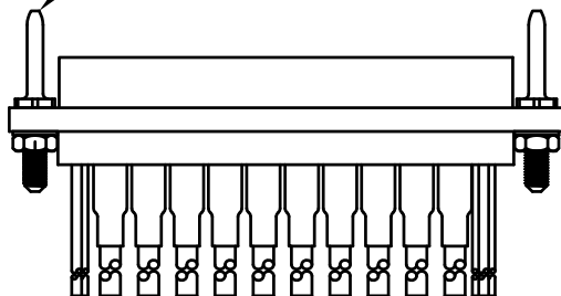
MR20P5S WITH BLIND MATE GUIDE PINS
