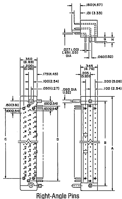
MIL-C-55302/7
