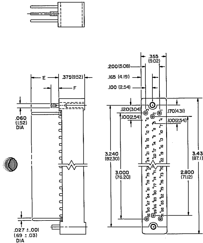
Straight-Thru Sockets
