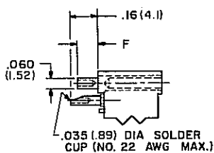
Solder Cup
