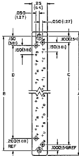
Straight-Thru Sockets
