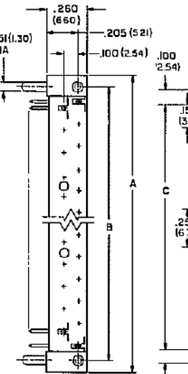
Right-Angle Pins
