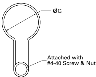
Split Retaining Ring
