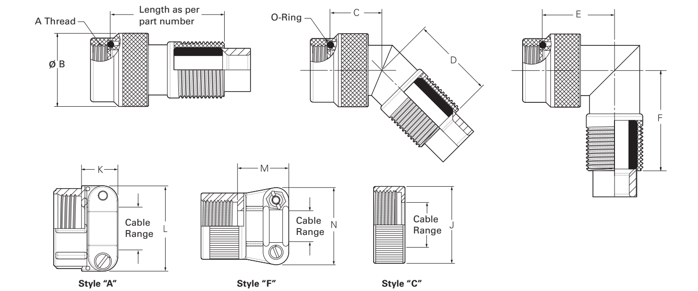
Backshell size codes and dimensions
