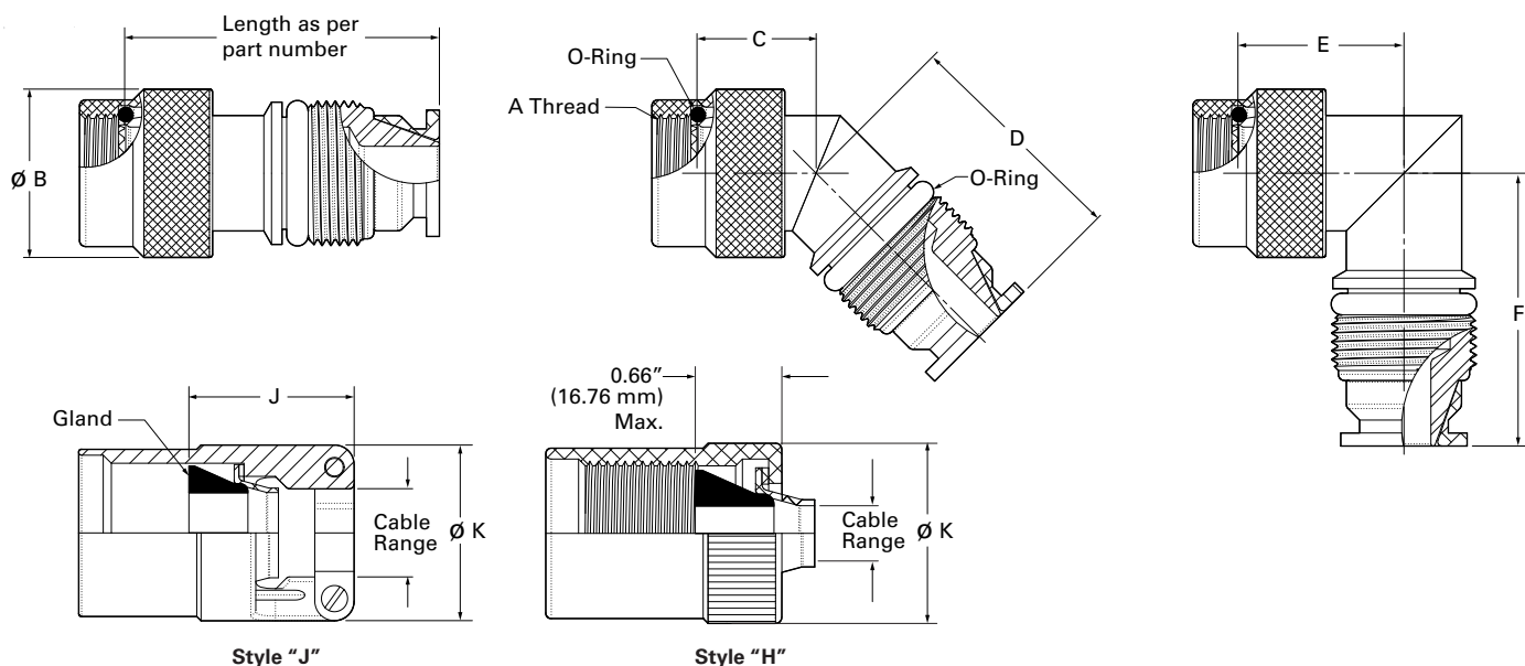
Backshell size codes and dimensions
